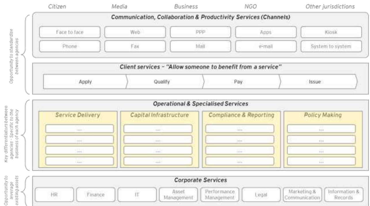
Figure 7: Operational Architecture to support analysis of Cloud adoption opportunities
