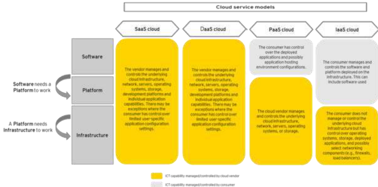
Figure 2: IT capability distribution within Cloud service models
