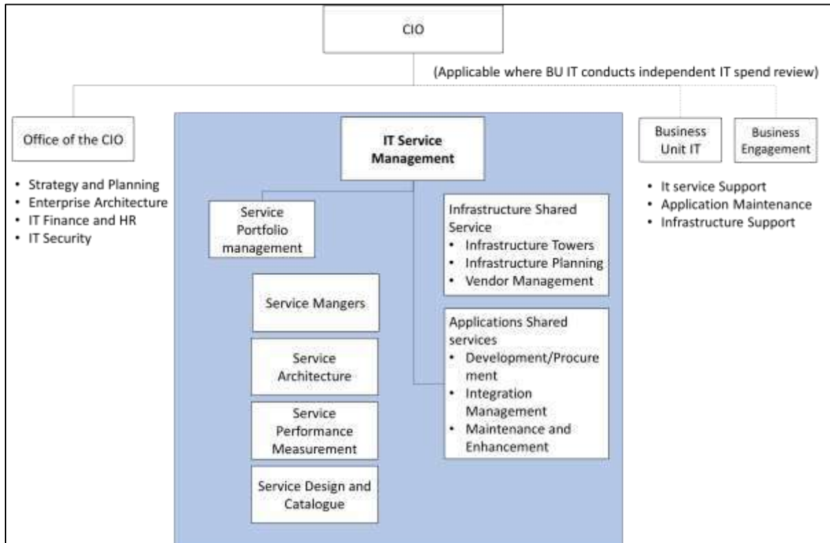
Figure 6: IT Service Management Organization target operating model
